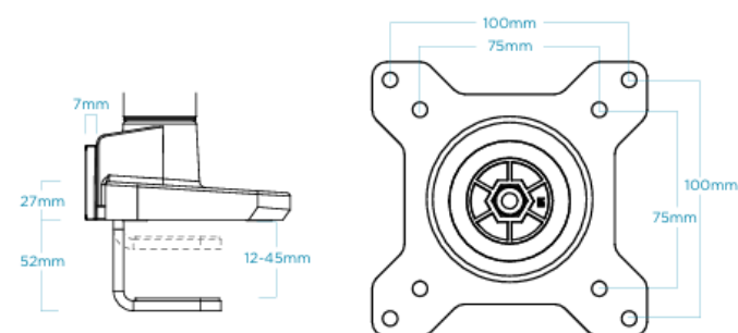
Arm Details
